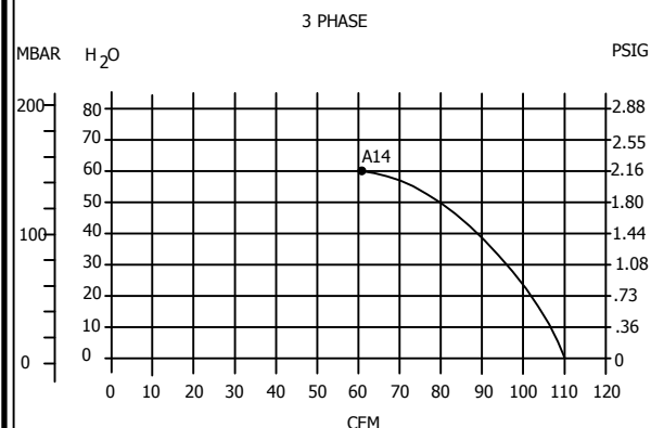
PRESSURE PERFORMANCE CURVE
