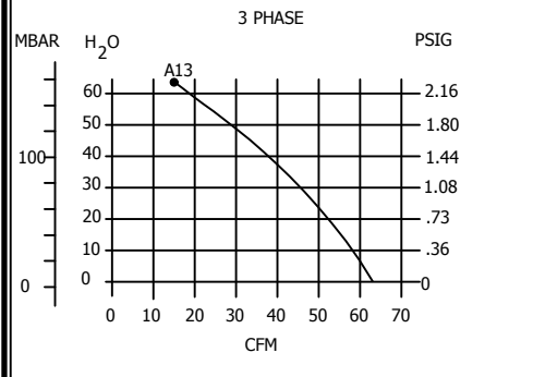
PRESSURE PERFORMANCE CURVE
